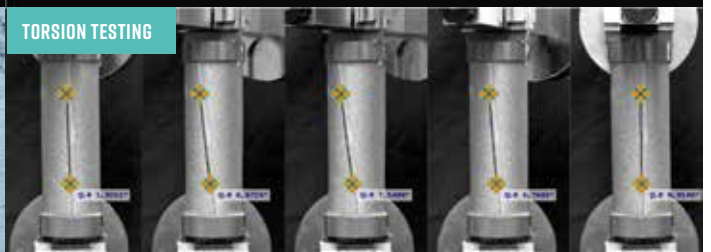
CRACK PROPAGATION
