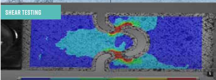
CRACK PROPAGATION
